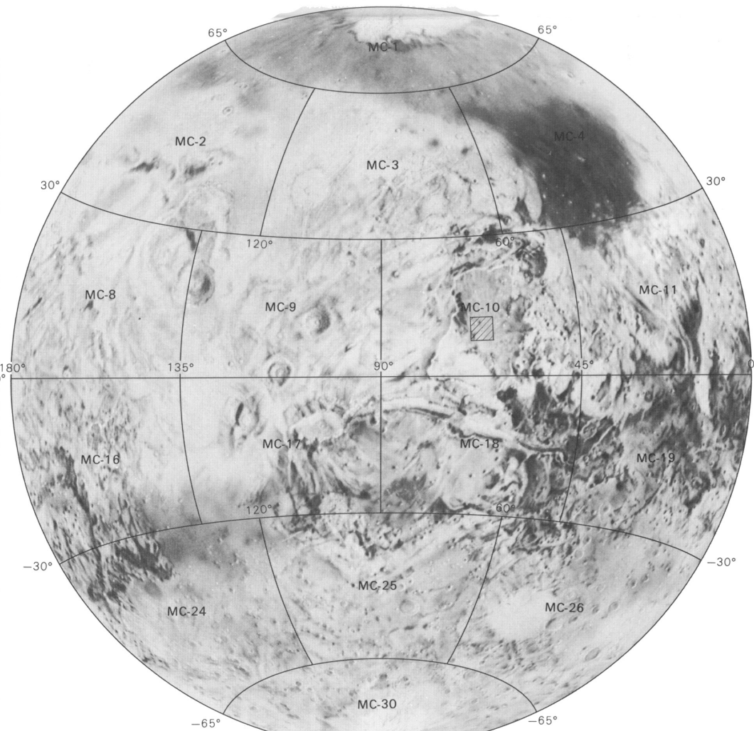
QUADRANGLE LOCATION Photomosaic location is shown in the western hemisphere of Mars. An outline of 1:500,000-scale quadrangles is provided for reference.
