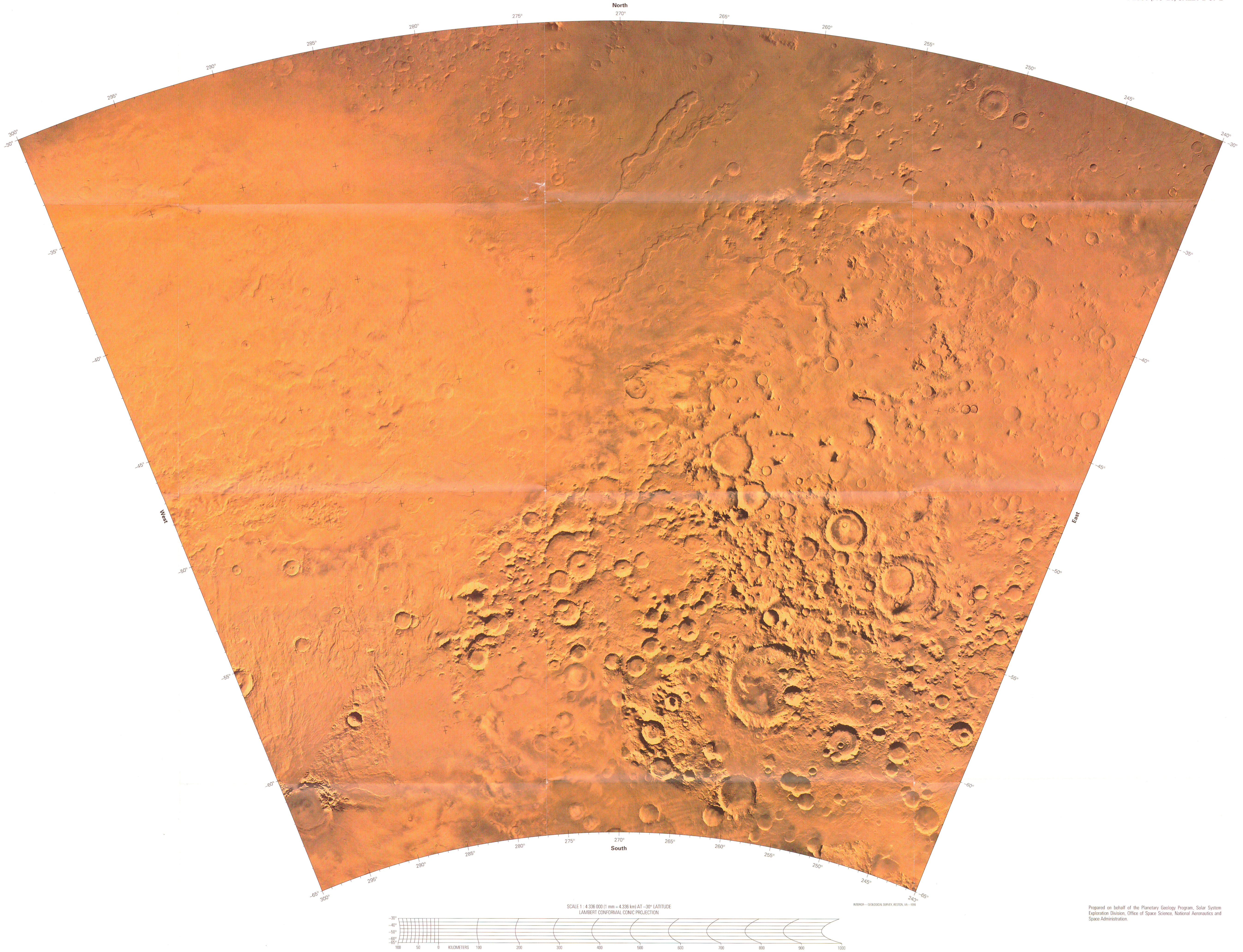
CONTROLLED COLOR PHOTOMOSAIC OF THE HELLAS QUADRANGLE (MC-28) OF MARS 1996
