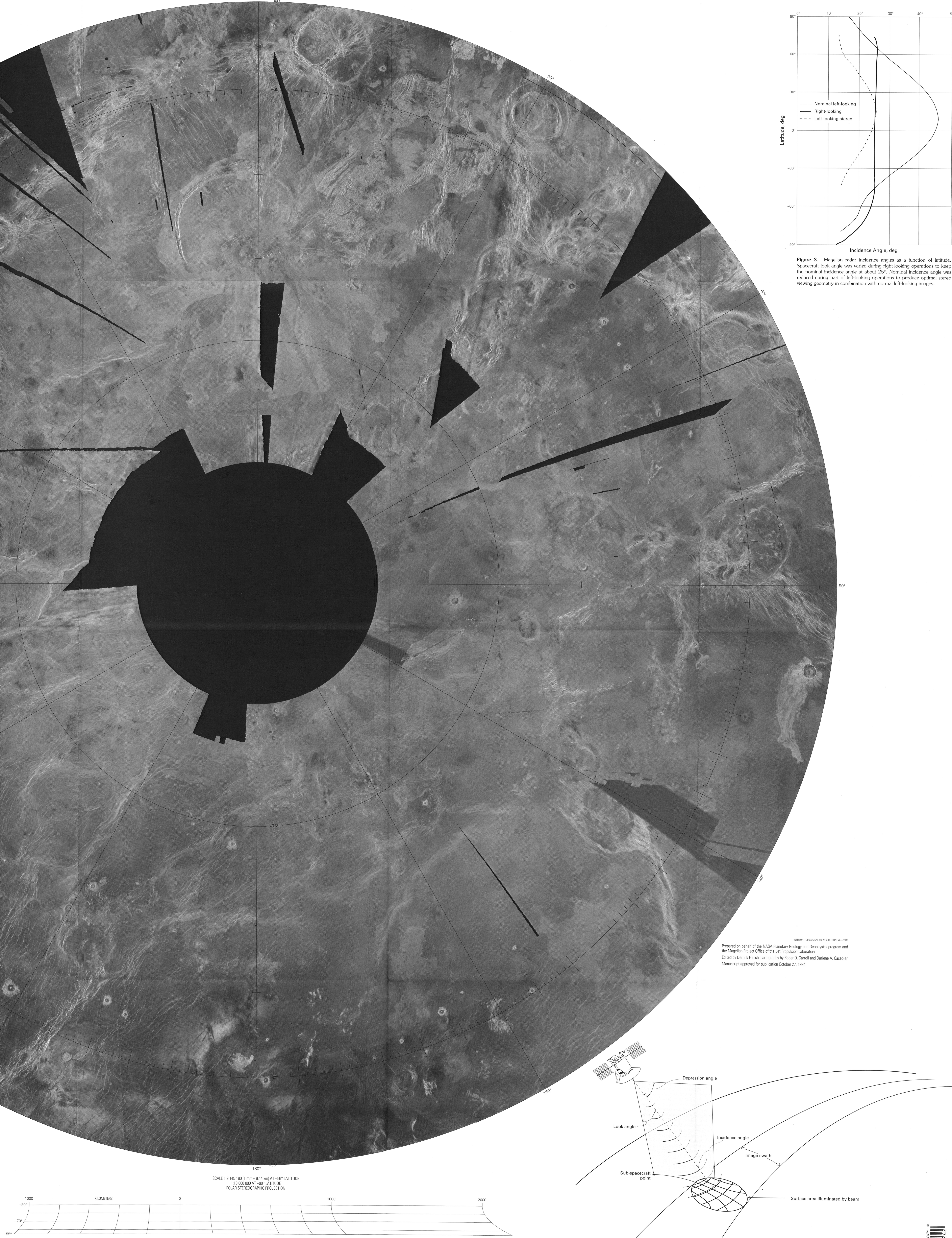
RADAR IMAGE MAP OF THE LADA TERRA REGION OF VENUS V 10M -90/0 CM 1998
