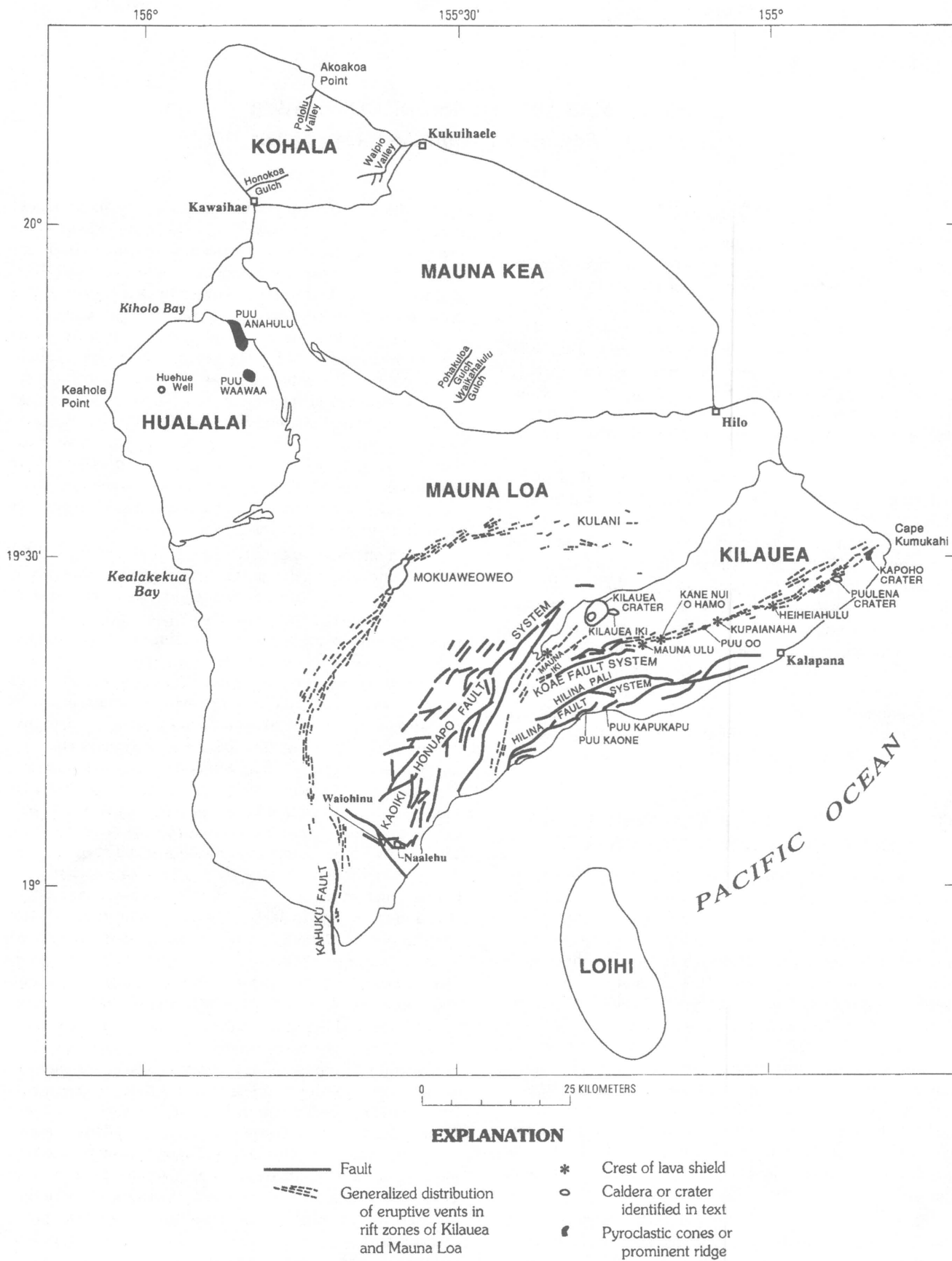
Figure 1. Map showing the five subaerial volcanoes (Kohala, Hualalai, Mauna Kea, Mauna Loa, and Kilauea) that form the Island of Hawaii and submarine Loihi Volcano forming on Hawaii's southeast flank.
