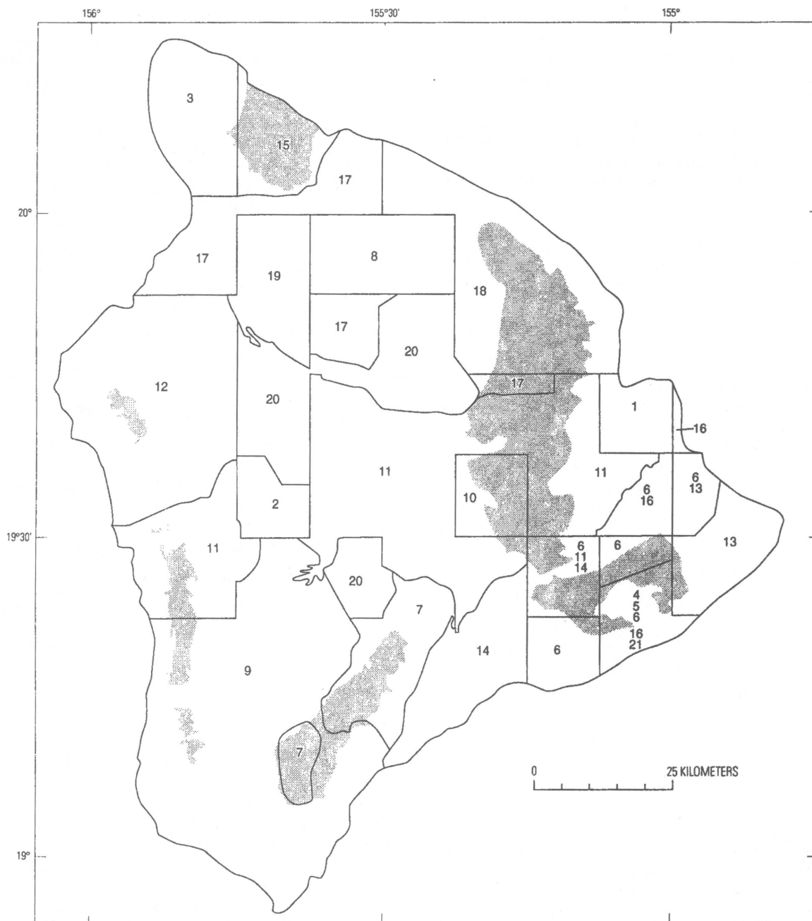
Figure 4. Sources of geologic mapping. In addition, critical information about age and distribution of historic lavas came from previously published geologic maps of the summits of Kilauea (Peterson, 1967) and Mauna Loa (Macdonald, 1971) and the middle part of the east rift zone of Kilauea (Moore and Koyanagi, 1969). Shading (modified from Jacobi, 1990) shows areas of exceptionally difficult access and visibility owing primarily to dense vegetation in both forest canopy and ground cover.
